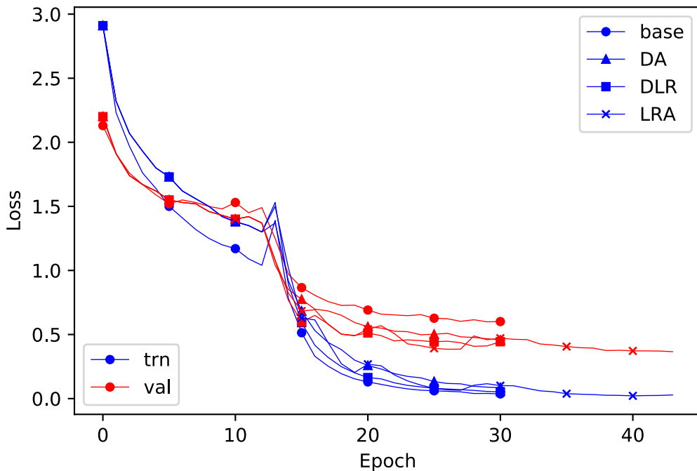
This figure shows the loss of each ResNet-50 model on the training set (trn) and validation set (val). The ResNet-50 models are: Transfer Learning and fine-tuning (base); base with data augmentation (DA); DA with differential learning rates (DLR); and DLR with learning rate annealing (LRA).
